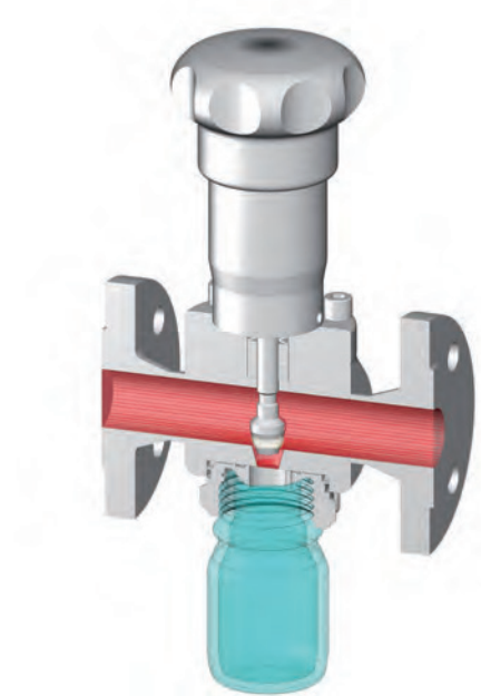
Principle of conical seat
